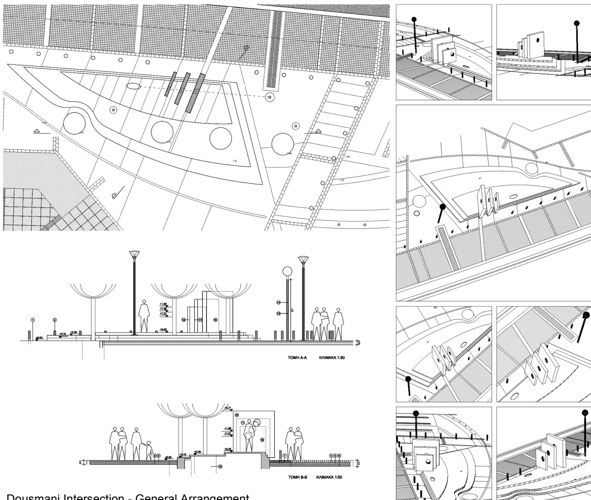
Dousmani Intersection - General Arrangement
